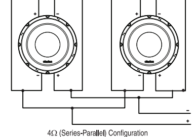
4Ω (Series-Parallel) Configuration
