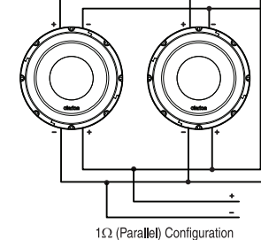
1Ω (Parallel) Configuration
