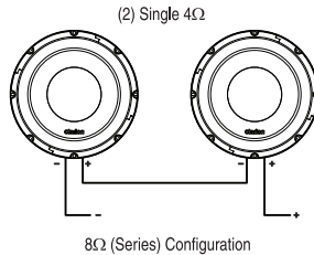
8Ω (Series) Configuration
