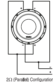
2Ω (Parallel) Configuration
