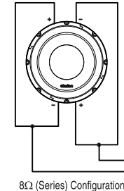
8Ω (Series) Configuration
